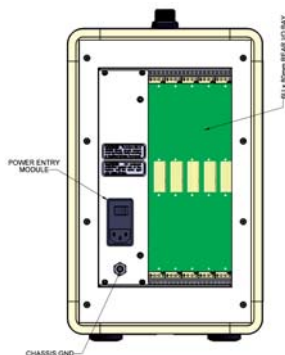
Series 815 full 6U x 80MM plug-in rear I/O
